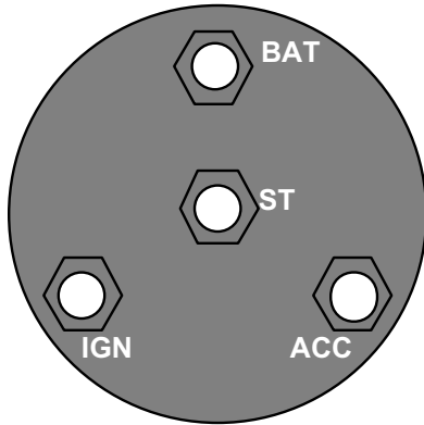
TYPICAL ICONNECTION (GM color coded)
