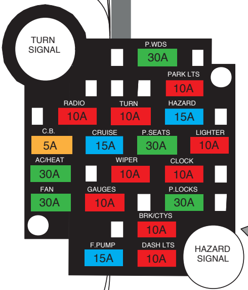
Fuse panel SEE SHEET 2
