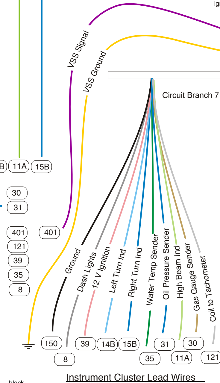
Circuit Branch 7 - Instrument Cluster Wiring
