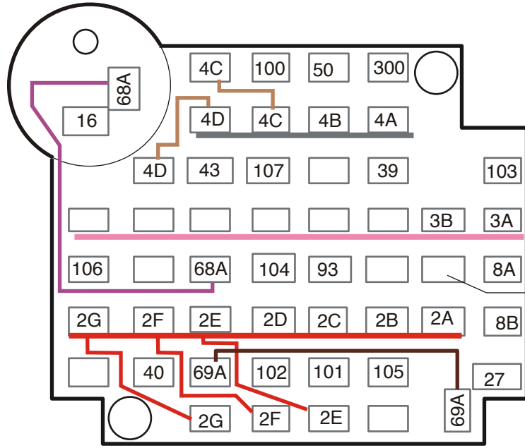
Fuse Box Connections (viewed from underside)
