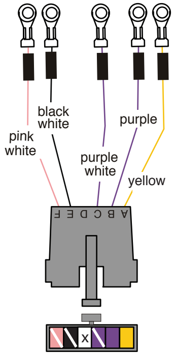
CONNECTOR C
