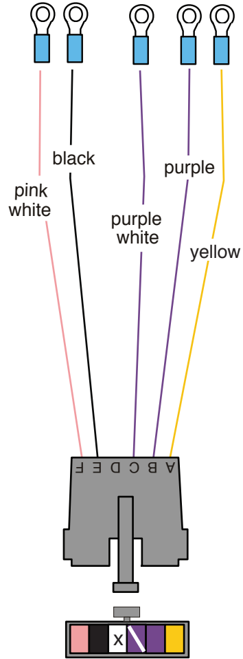
CONNECTOR C
