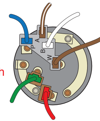
1970-71 variable-speed wiper switch
