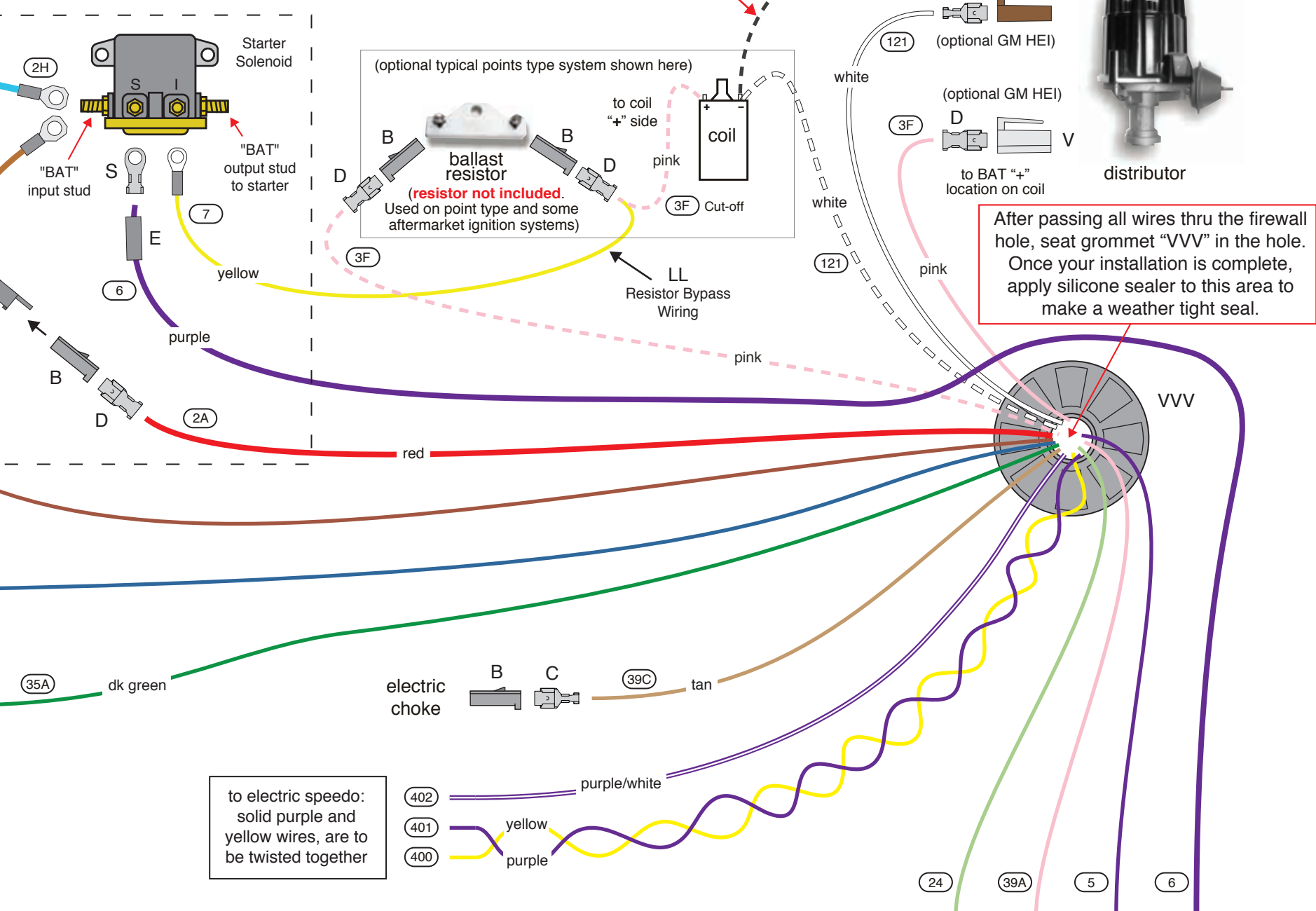
Figure "II" Ignition, engine sensors, electric choke, tachometer, electric speedometer, alternator, back-up switch and NSS
